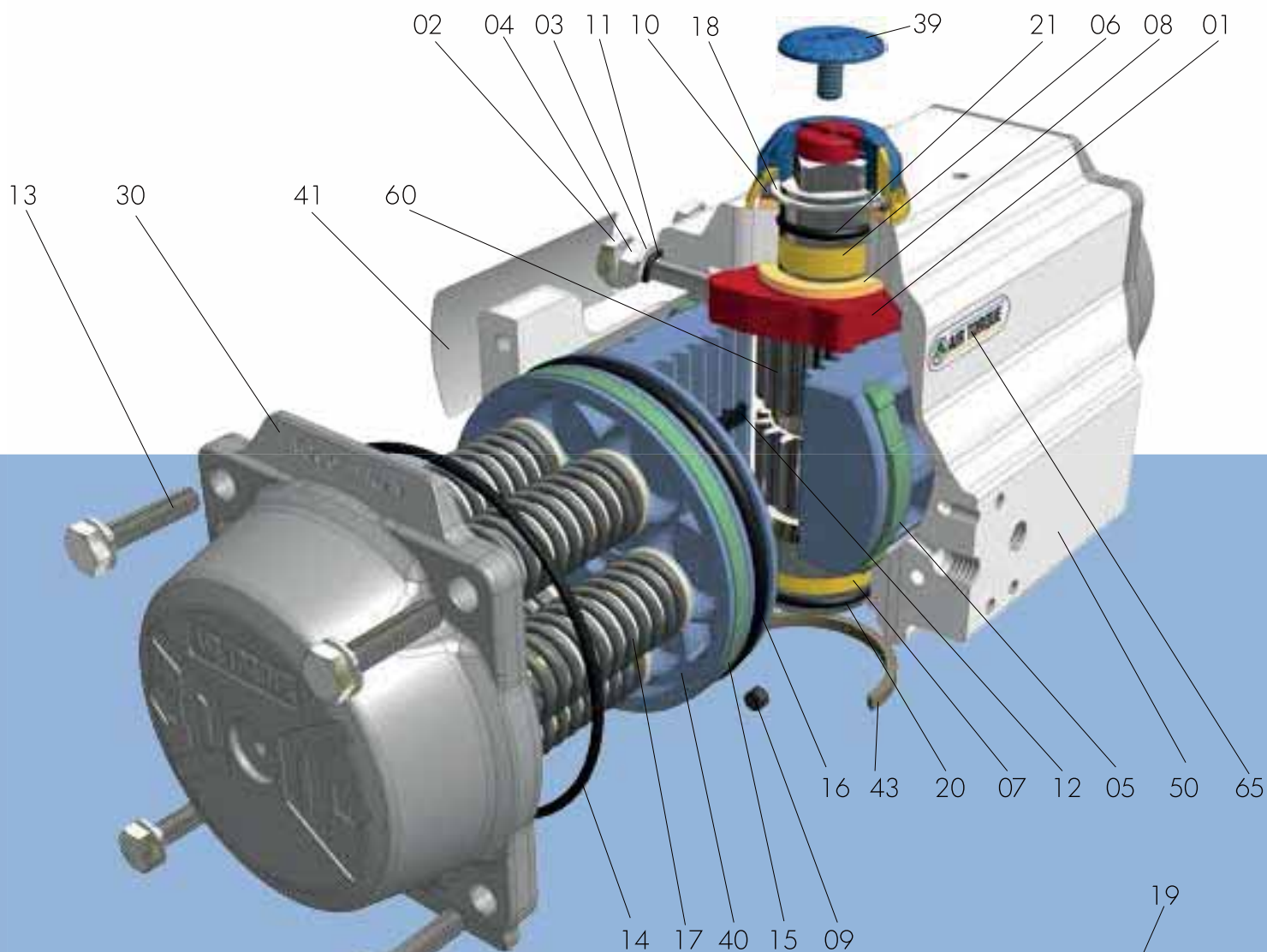
Spring for AT045U ÷ AT051U
